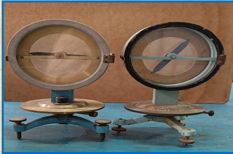
DIP CIRCLE
