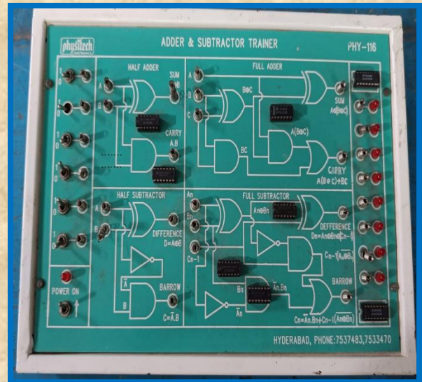
ADDER & SUBTRACTOR TRAINER KIT
