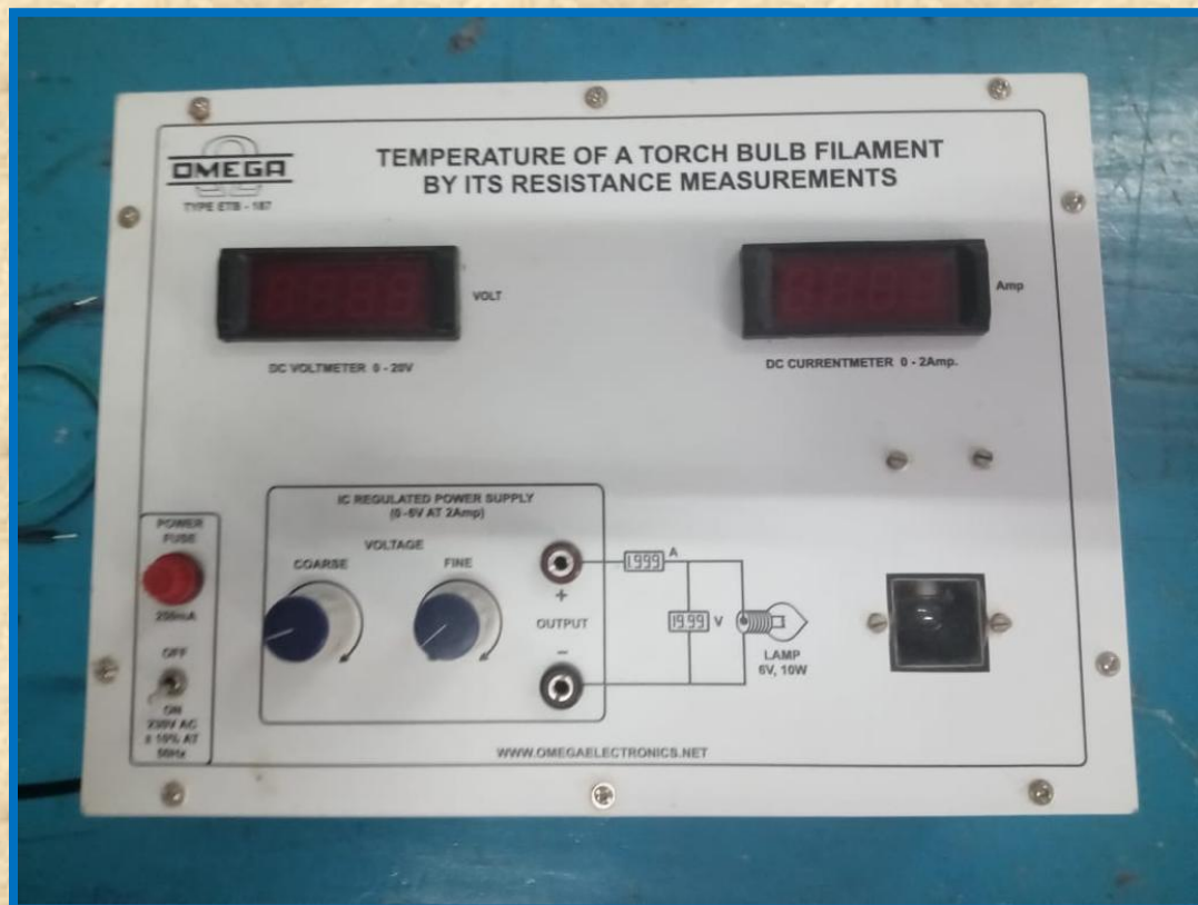
ELECTRICAL BULB CHARACTERISTICS TRAINER
